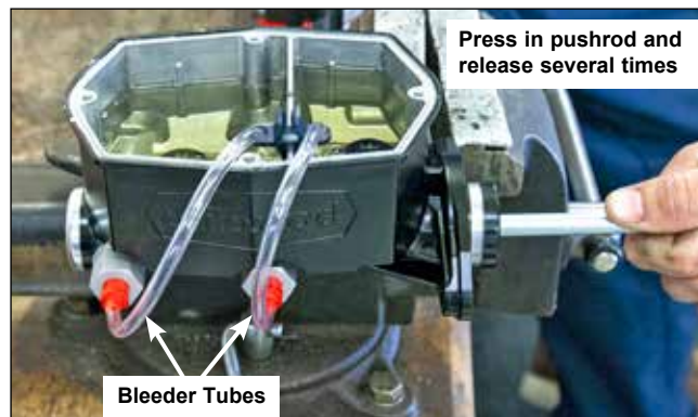
Typical Bleeder Tube Setup and Use
