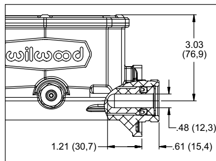
Master Cylinder Piston Detail P/N's 260-14959/60
